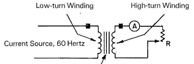
Current Transformer to be Demagnetized
