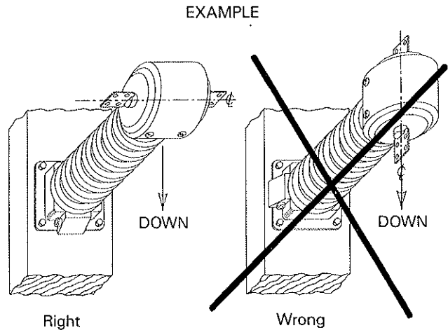
Fig. 3. Examples of right and wrong CT mounting
