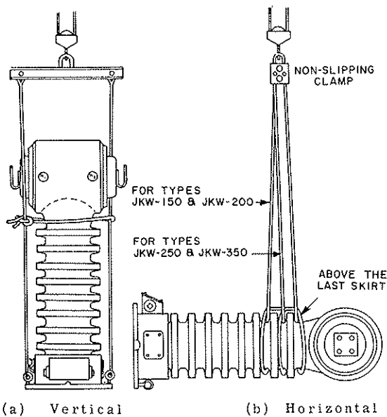
Fig. 2. Method of lifting transformers
