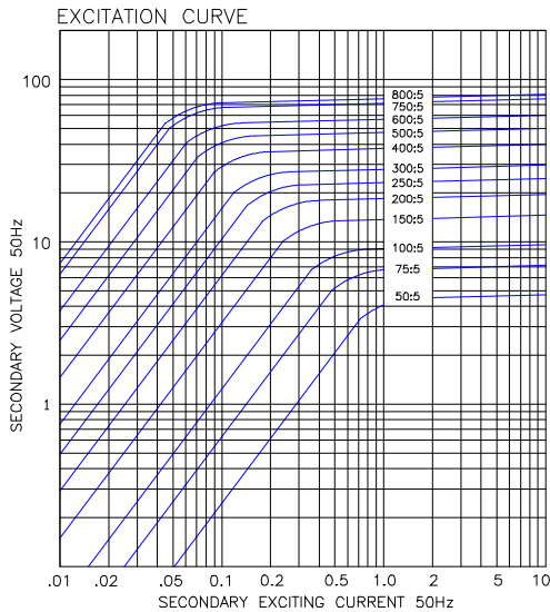
Model 299I Window Diameter 85.9mm Approximate weight 4.5 kg
