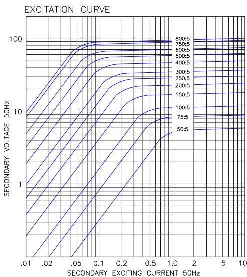
Model 298I Window Diameter 76.2mm Approximate weight 5.4 kg
